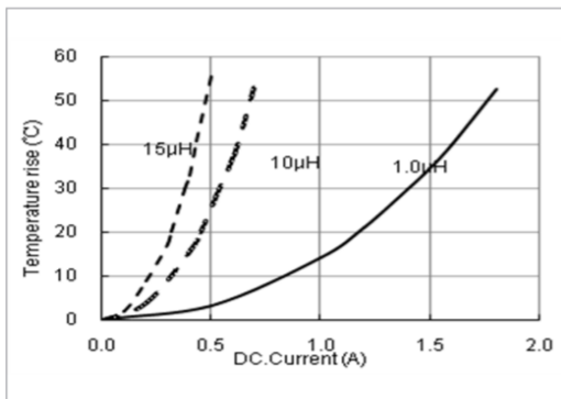
SWPA252012S Series Temperature vs. DC Current Characteristics
