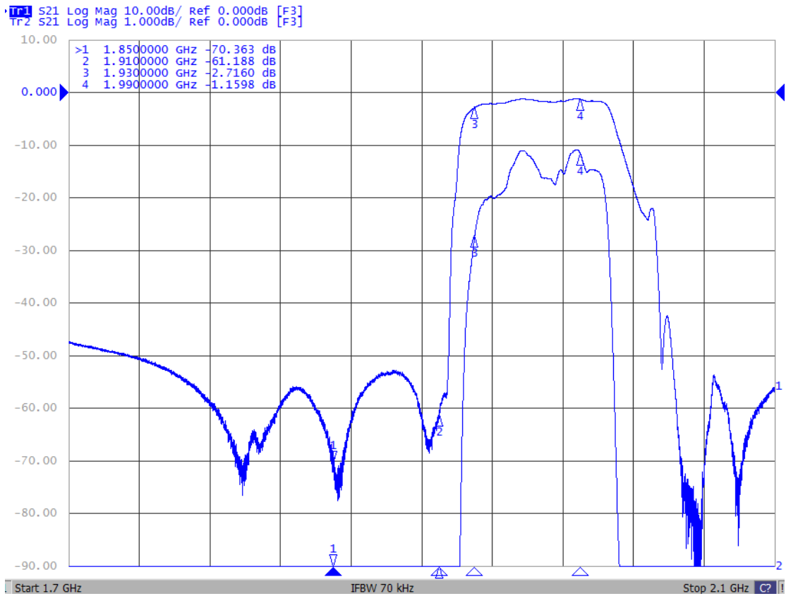
Figure 8: ANT→RX
