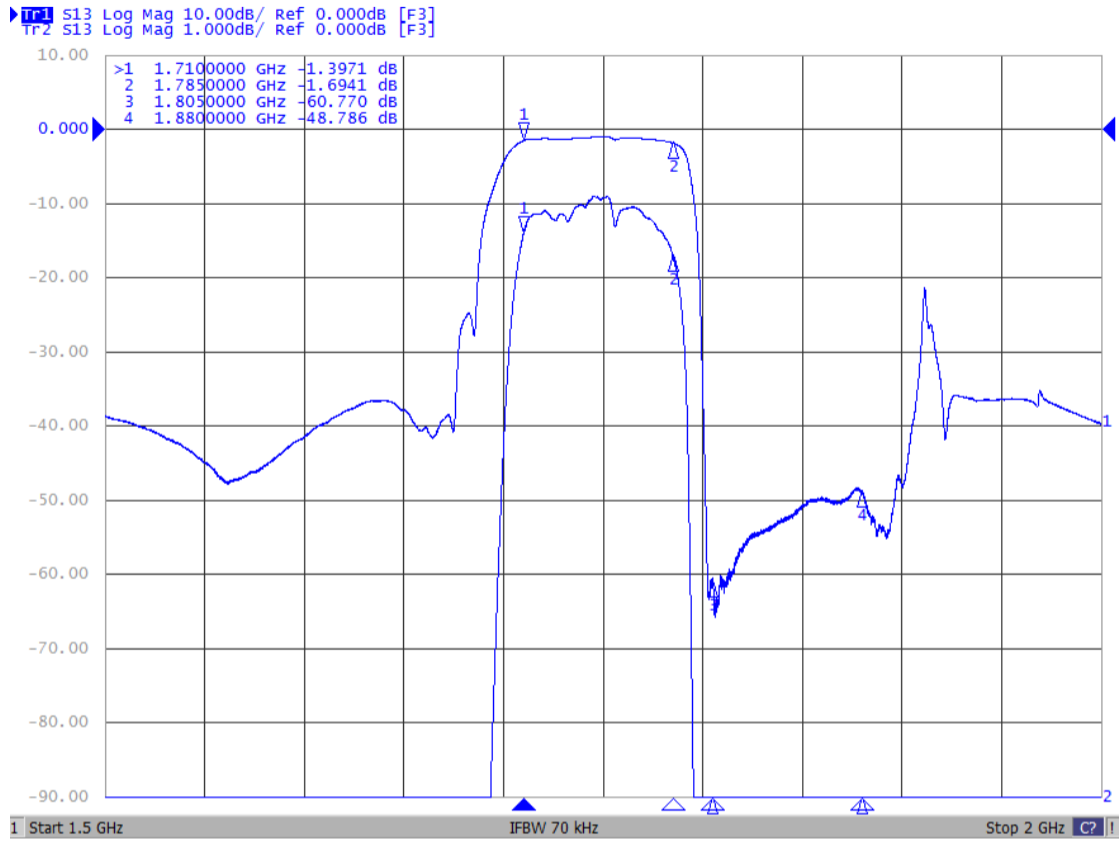
Figure 4: TX→ANT
