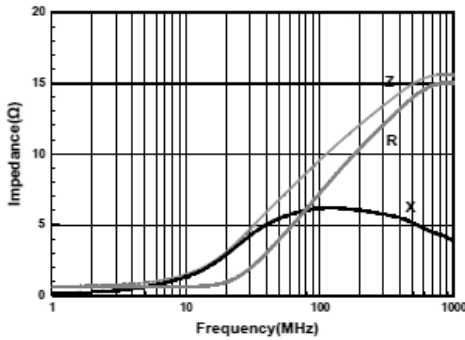
SBH1005S100PSP
