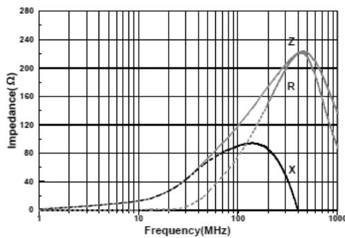
SBH1005S601JSP
