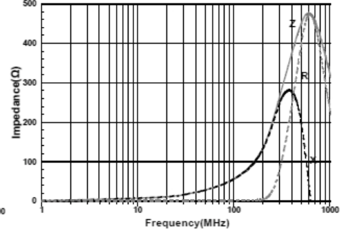
SBH1608S181MSP
