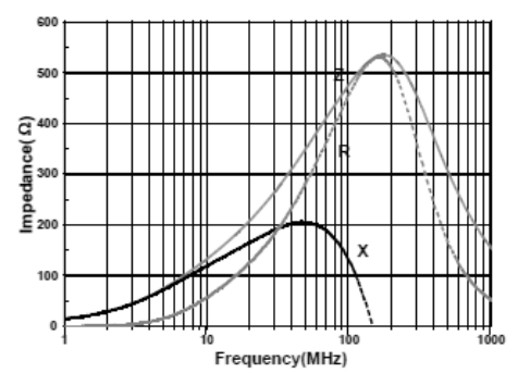
SBH1608S152FSP
