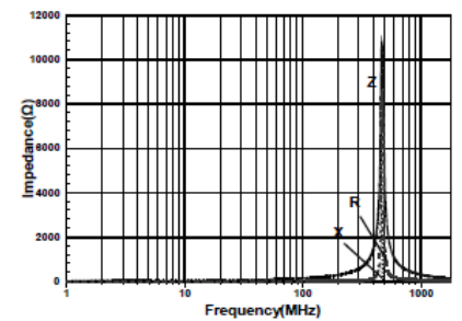
SBM1608G331GSP
