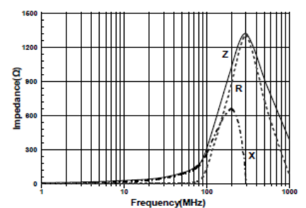
SBM1608G331GSP
