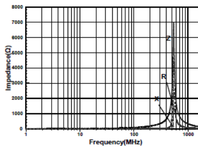
SBM1608G221GSP
