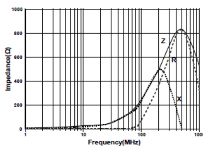
SBM1608G221GSP
