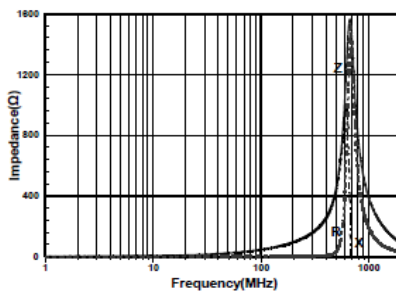
SBM1608G121HSP
