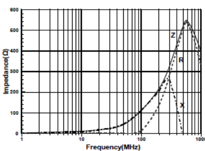
SBM1608G121HSP
