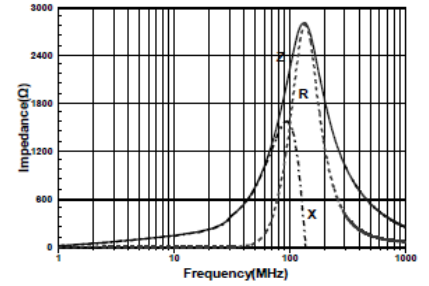
SBM1608K222BSP
