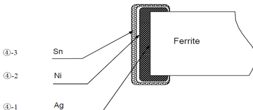
Fig.2 Body Structure
