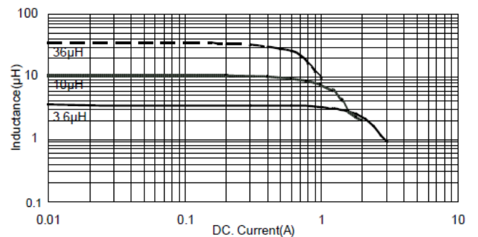
Inductance vs. DC Current Characteristic
