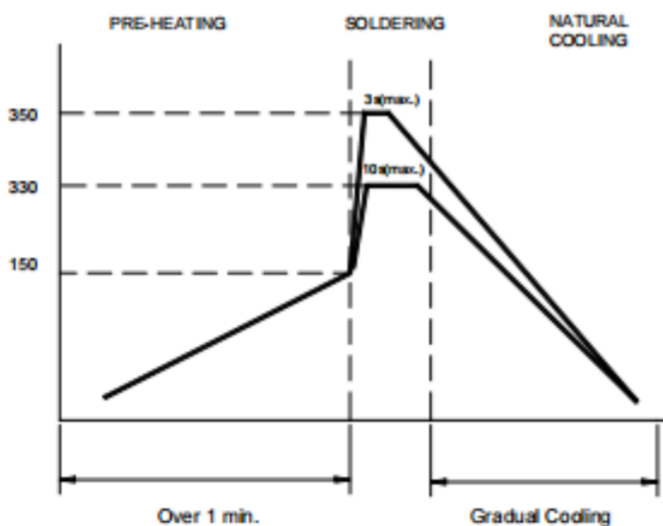
Figure 2. Hand Soldering
