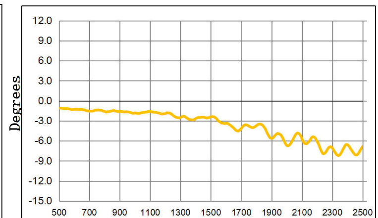
Phase Balance
