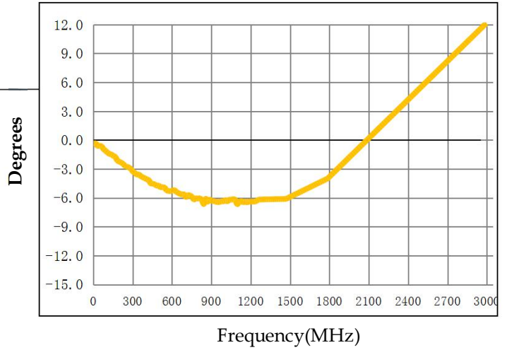
Phase Balance
