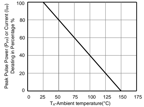
Figure 2 -Pulse DeratingCurve
