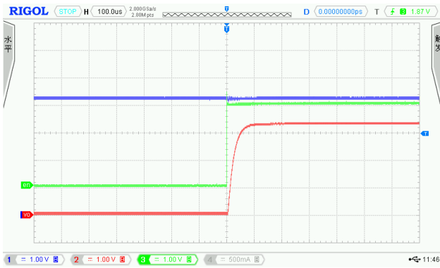
EN=0V to 3V, I OUT =10mA
