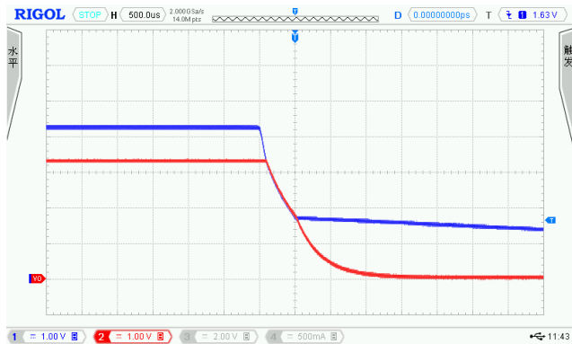
V IN =4.3V to 0V, I OUT =10mA
