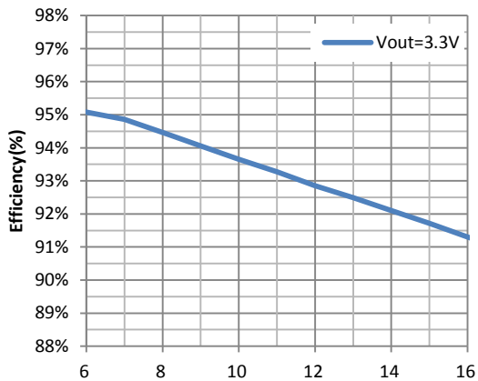
Efficiency vs. Vin Iout=1A
