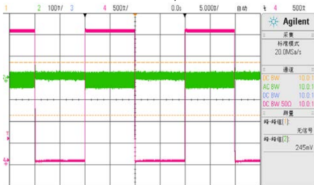
Load Transient
