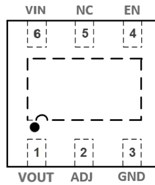
DFN2020-6 ADJ Pin Configuration
