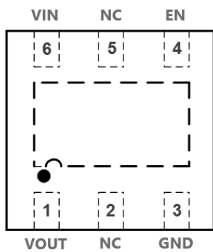
DFN2020-6 Fixed Pin Configuration
