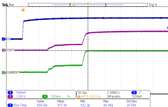
SUL6001D8-33
