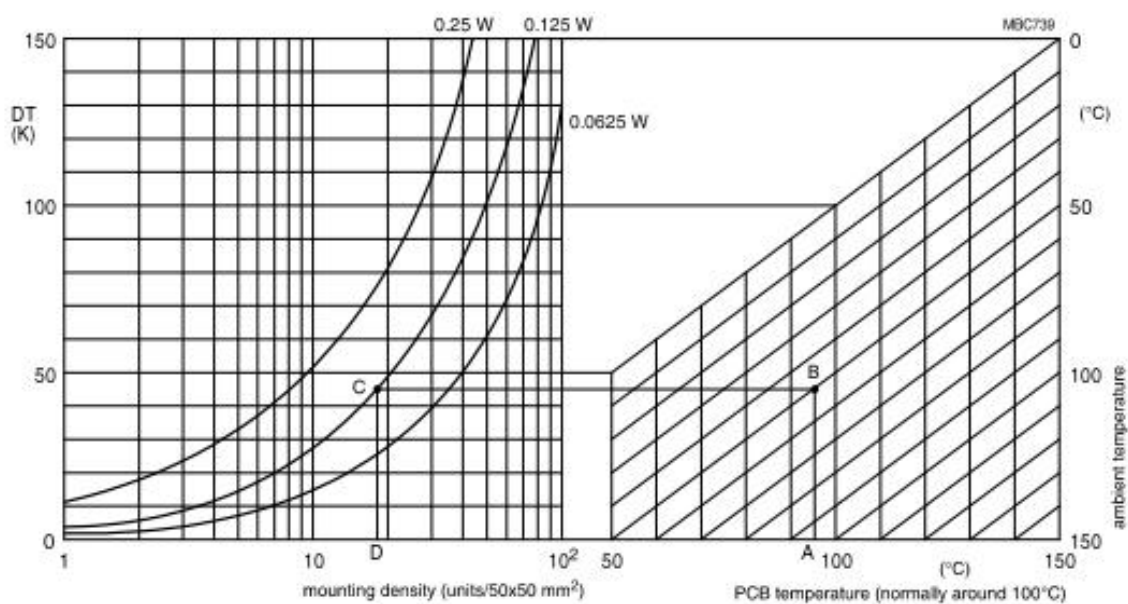
Fig5: PCB temperature as a function of applied power, mounting density ambient temperature
