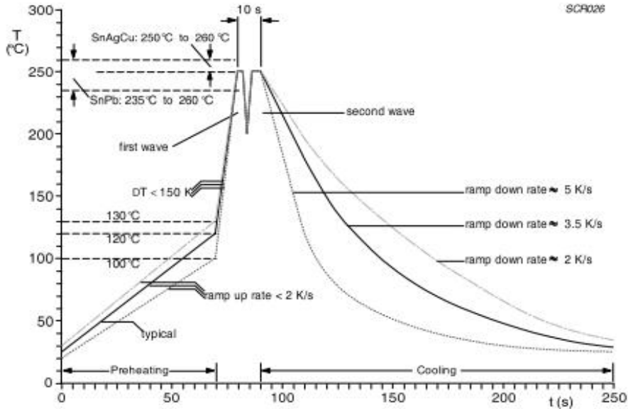
Fig8: Double wave soldering for SnPb and leadfree SnAgCu solder-temperature/time profile (terminal temperature)
