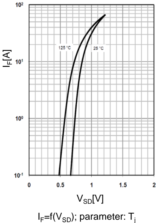
Forward characteristics of reverse diode
