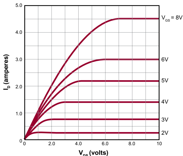
Saturation Characteristics
