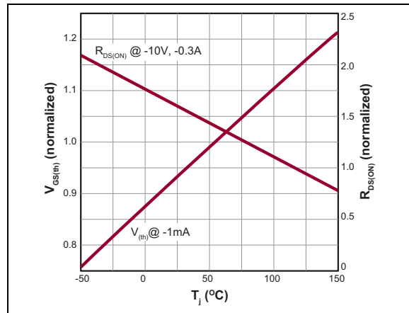
FIGURE 2-5: V_{GS(th)} and R_{DS} Variation with Temperature.
