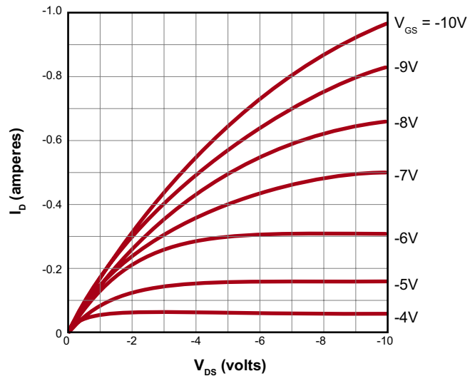
Saturation Characteristics
