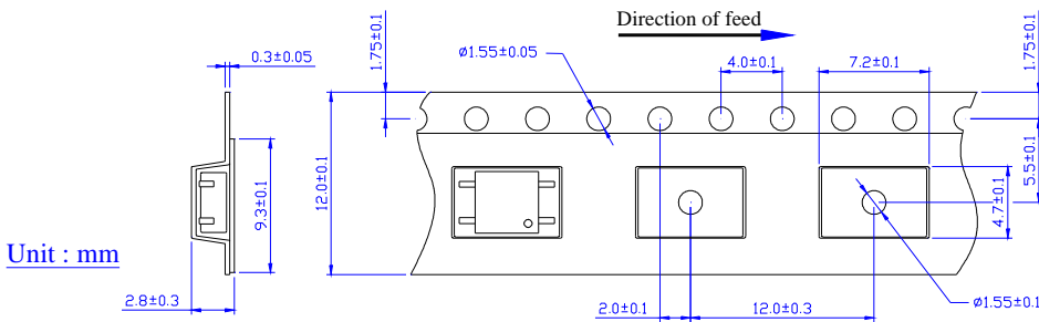
Tape dimensions
