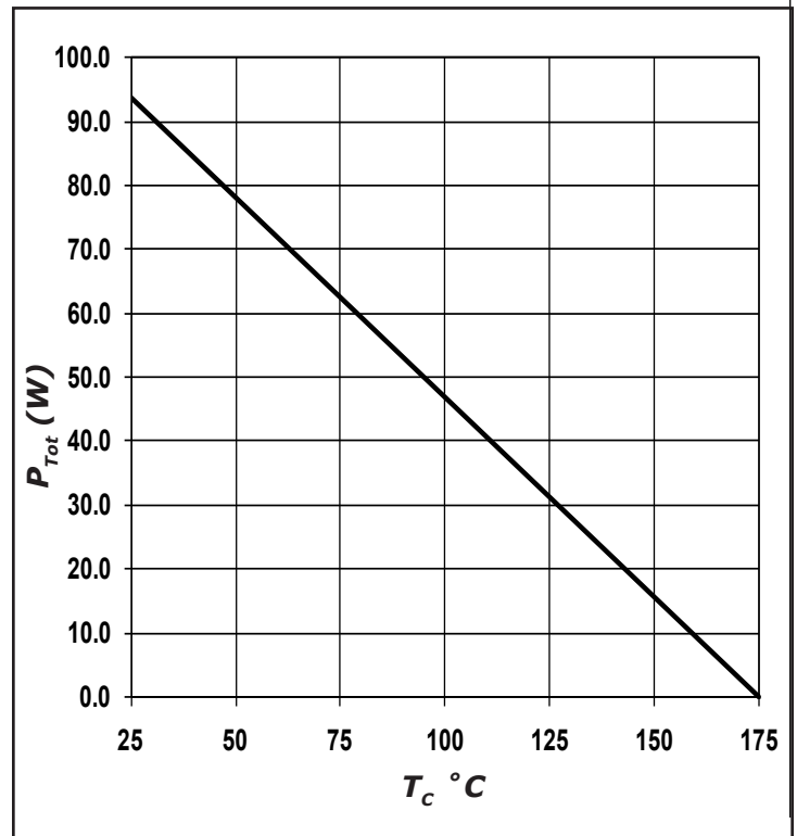
Figure 4. Power Derating
