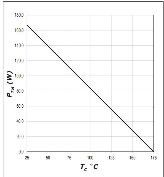
Figure 4. Power Derating
