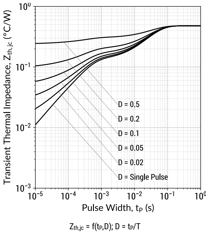
Figure 9: Transient Thermal Impedance (Per Leg)
