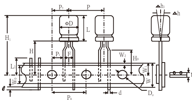
Fig.3( \phi 5-\phi 8 )
