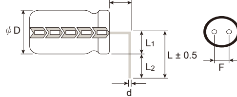
SHAPE (L)
