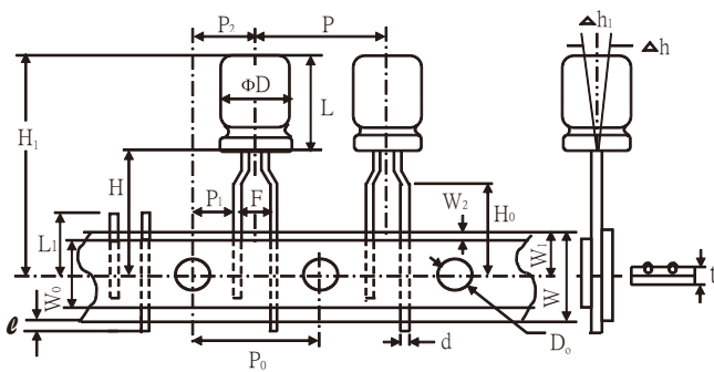
Fig.3( \phi 5-\phi 8 )
