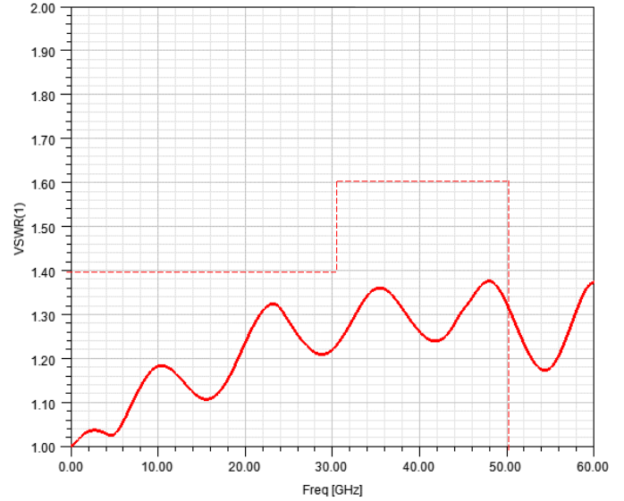
VSWR Plot 1.
