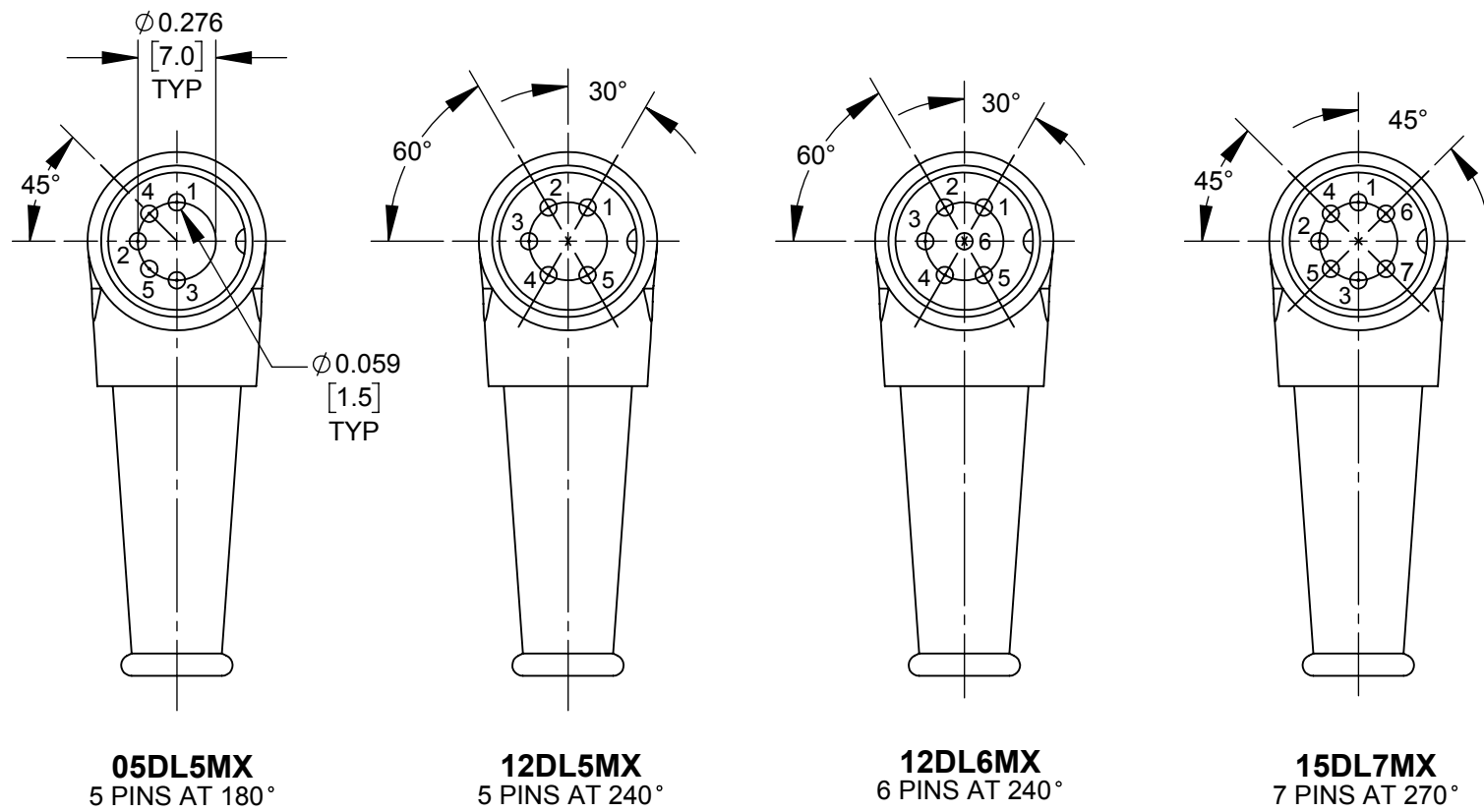
PIN LAYOUTS
