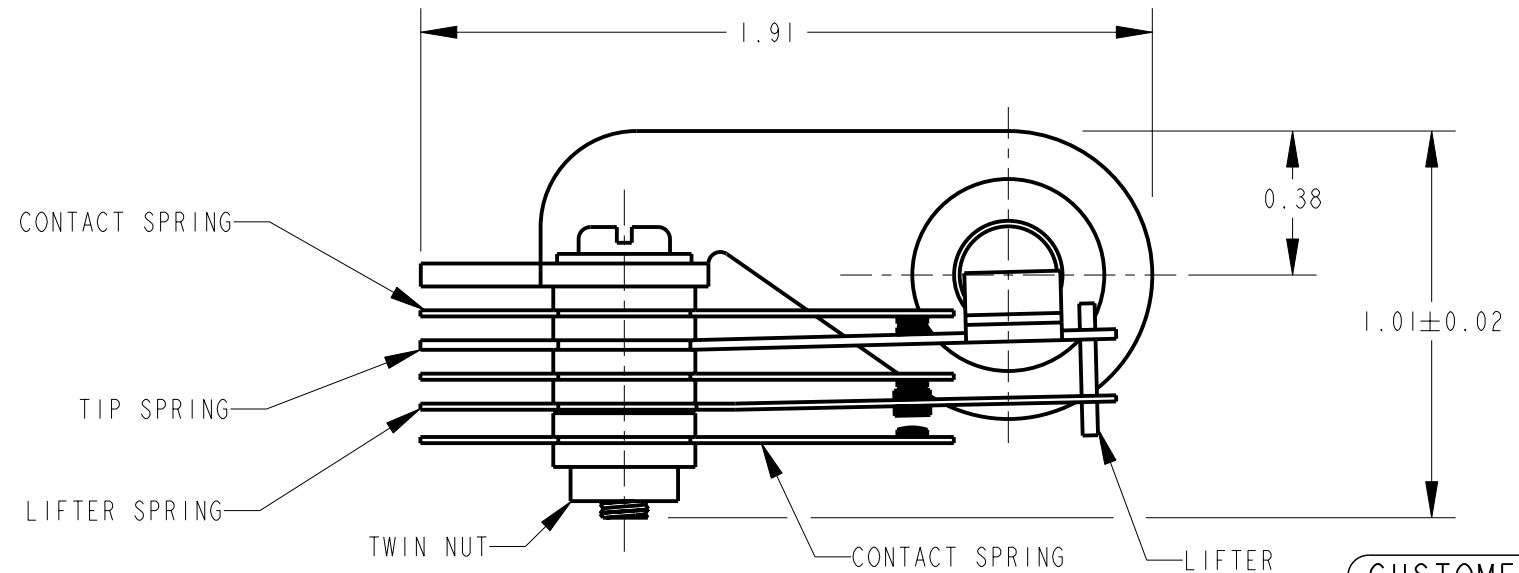
CUSTOMER DRAWING
