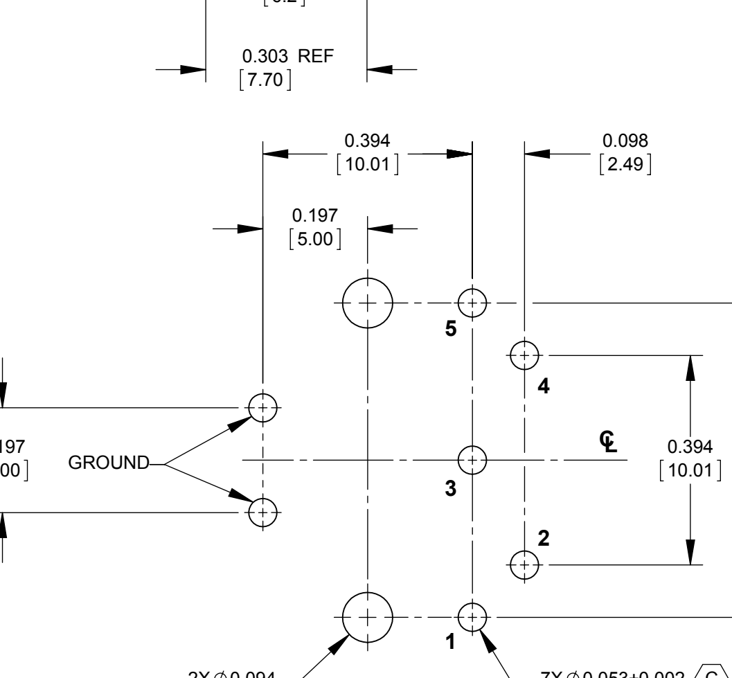
RECOMMENDED PC BOARD LAYOUT COMPONENT SIDE
