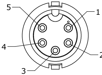
FACE VIEW 6280-5PG-5XX
