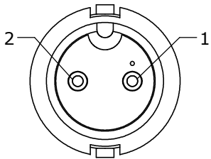
FACE VIEW 6280-2PG-5XX
