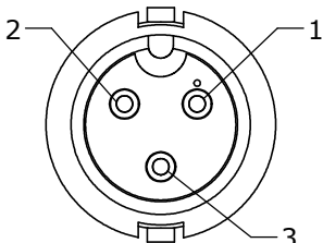
FACE VIEW 6280-3PG-5XX
