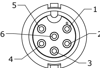
FACE VIEW 6280-6PG-5XX
