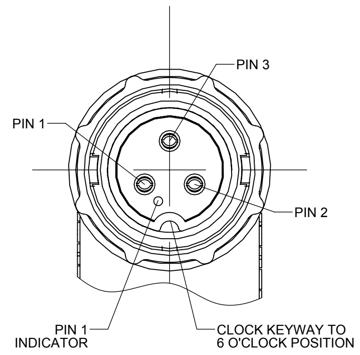
PIN CALLOUT VIEW FROM MATING SIDE OF CONNECTOR SCALE=3:1
