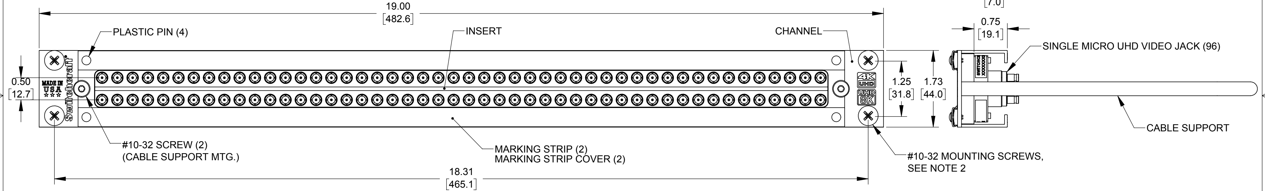
FRONT VIEW
