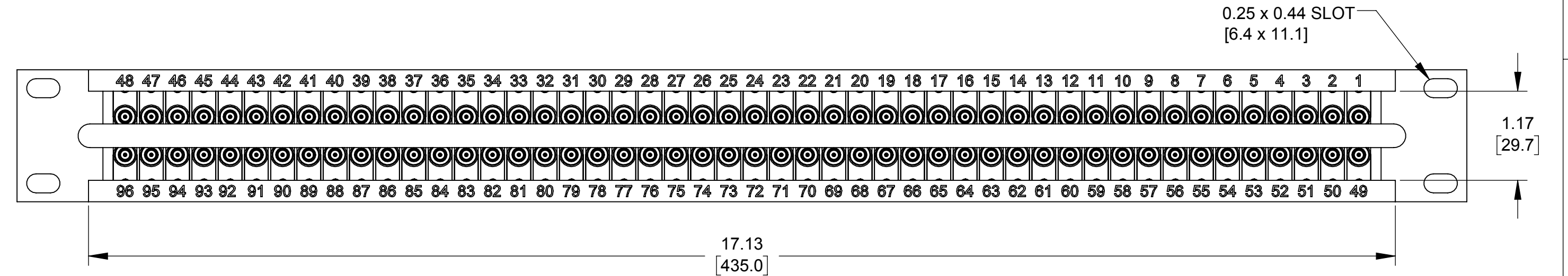
REAR VIEW
