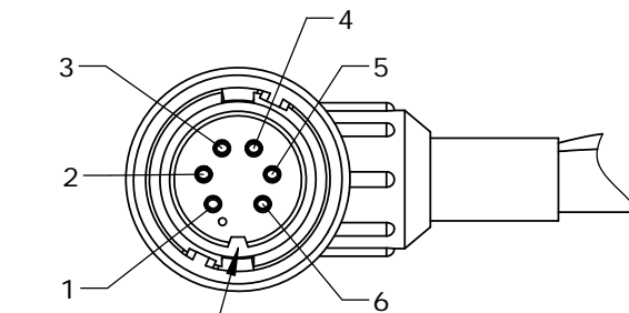
KEYWAY AT 9 O'CLOCK POSITION END "A" FACE VIEW
