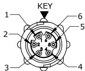
FACE VIEW W18980-6SG-P-5XX 6 POSITION
