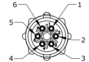
WIRING VIEW W18980-6SG-P-5XX
