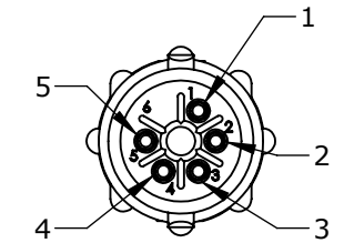
WIRING VIEW W18980-5SG-P-5XX
