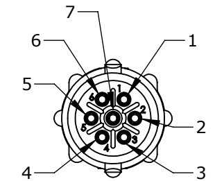
WIRING VIEW W18980-7SG-P-5XX
