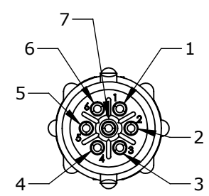
WIRING VIEW W18982-7SG-P-5XX
