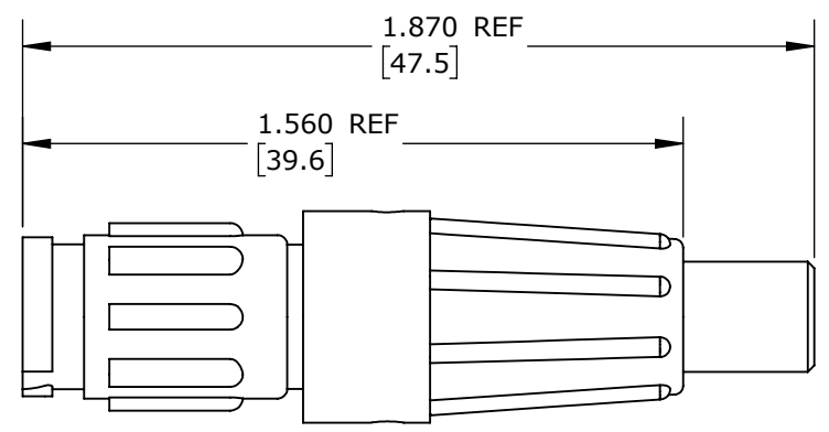
ASSEMBLED VIEW FOR CUSTOMER REF. ONLY
