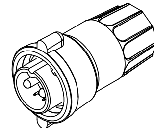
WINGED COUPLING RING P/N: W3B82-8PG-3XXW
