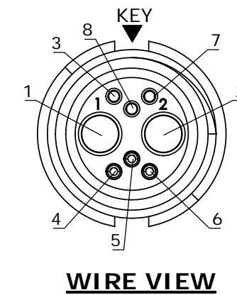
WINGED COUPLING RING P/N: W3B82-8PG-3XXW
