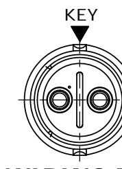
WIRING END W6380-2PG-P-3XX SHOWN WITHOUT HARDWARE
