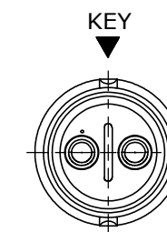
WIRING END W6382-2SG-P-5XX SHOWN WITHOUT HARDWARE
