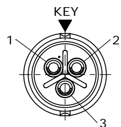
WIRING END W6382-3PG-P-3XX
