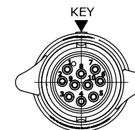
WIRING END ASSY: W6882-10SG-P-5XX SHOWN WITHOUT HARDWARE
