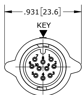
MATING FACE ASSY: W6882-10SG-P-5XX SHOWN
