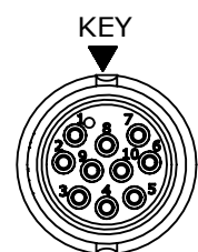
WIRING END W6882-10SG-P-5XX
