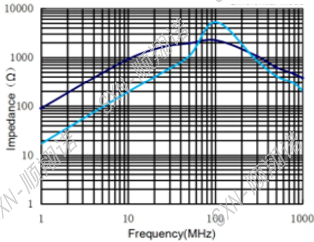
SMCM9070-222T
