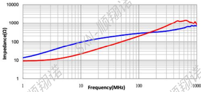
SMCM4520-701T
