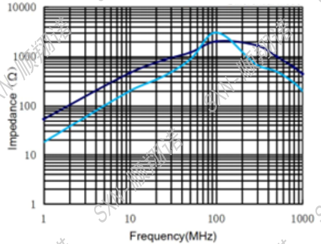
SMCM9070-272T
