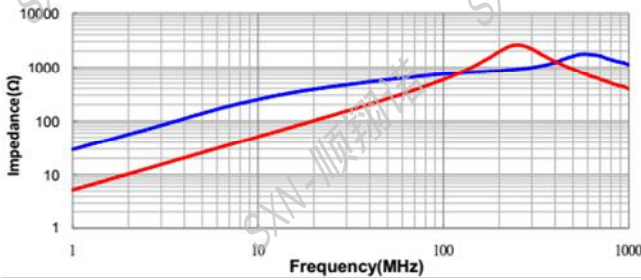
SMCM4520-701T
