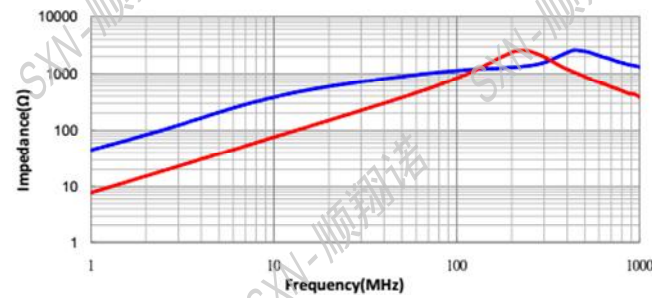
SMCM4520-122T
