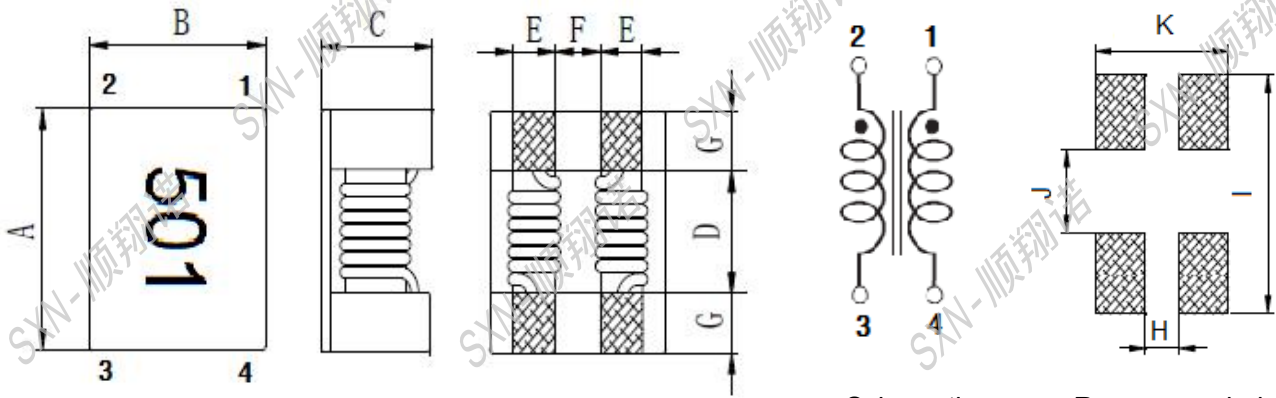
Schematic
