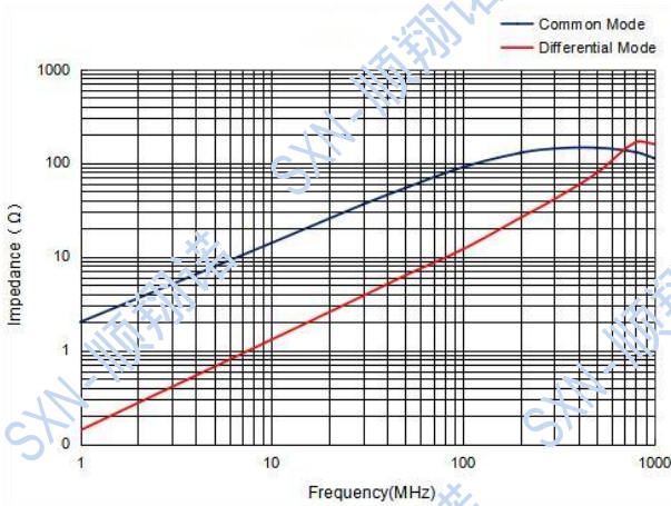
SMDCM5020-101T
