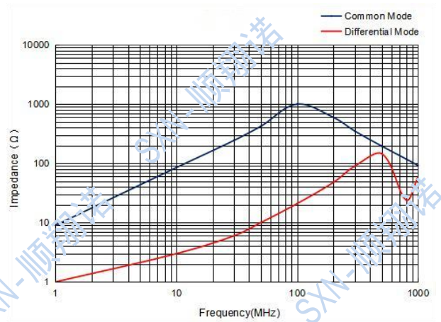
SMDCM5020-901t&102T
