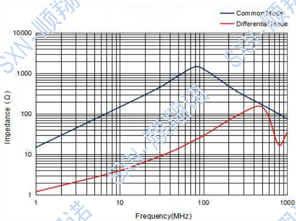
SMDCM5020-142T&152T
