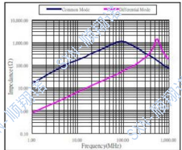
SMDCM5040-102T
