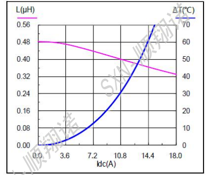
SMMS0530-R47M
