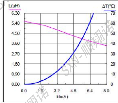
SMMS0630-5R6M
