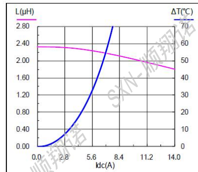
SMMS0530-6R8M
